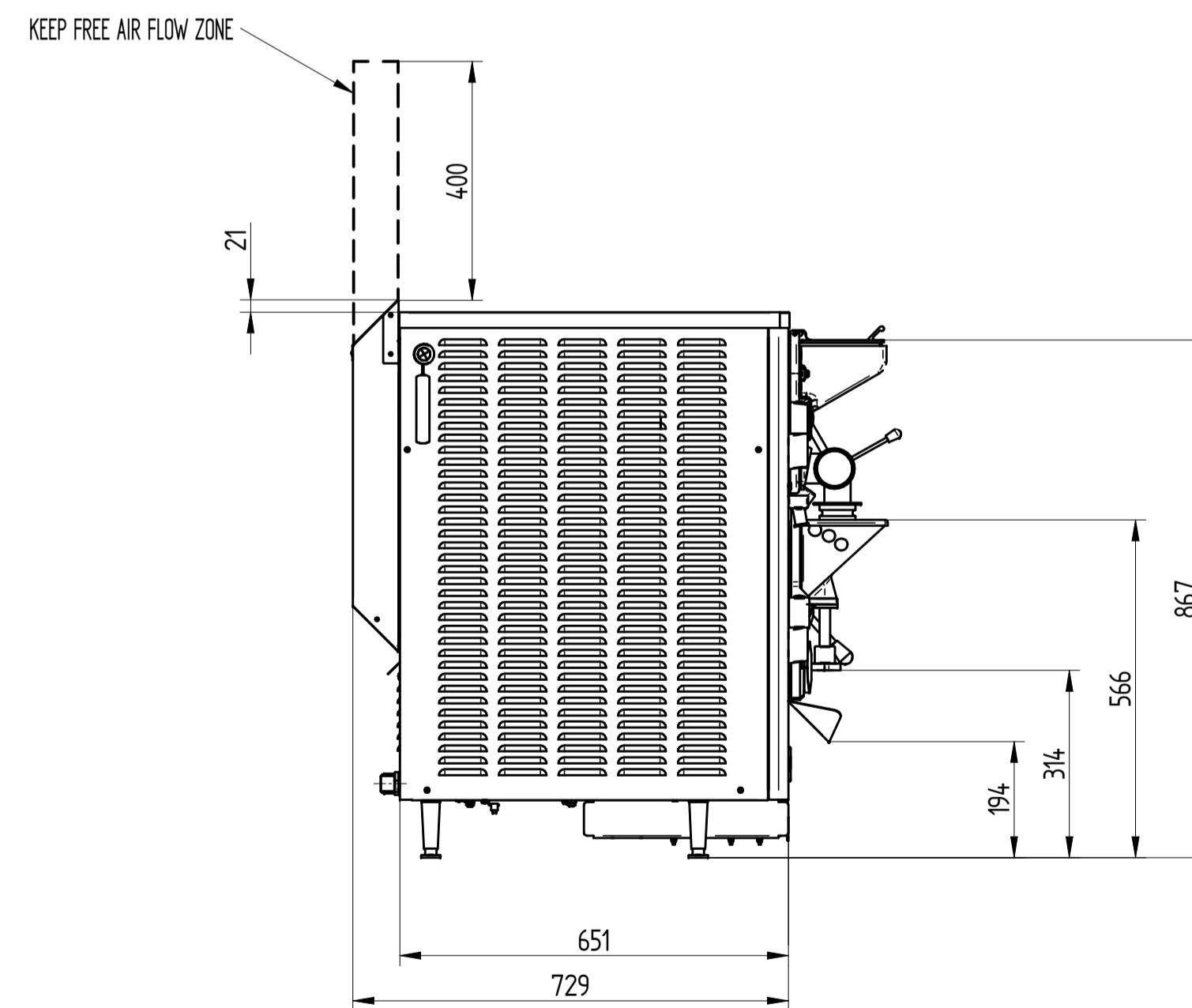
LEFT SIDE VIEW AIR VERSION
