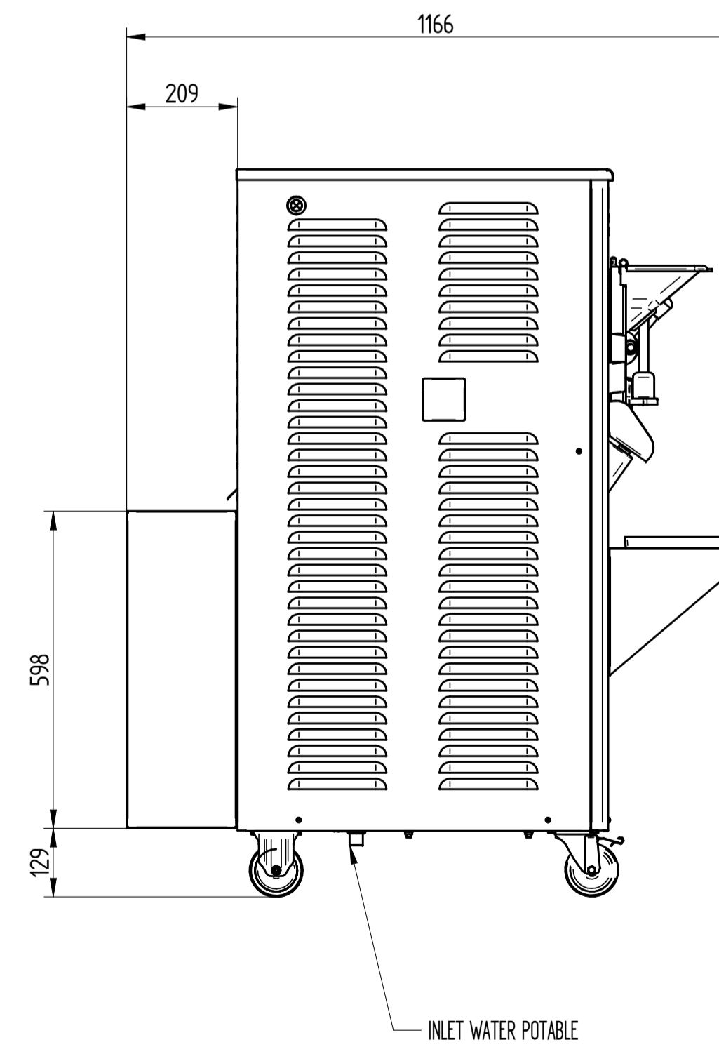
LEFT SIDE VIEW AIR VERSION
