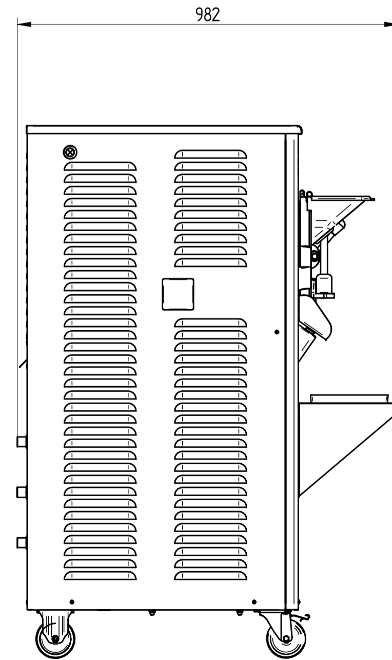
LEFT SIDE VIEW WATER VERSION
