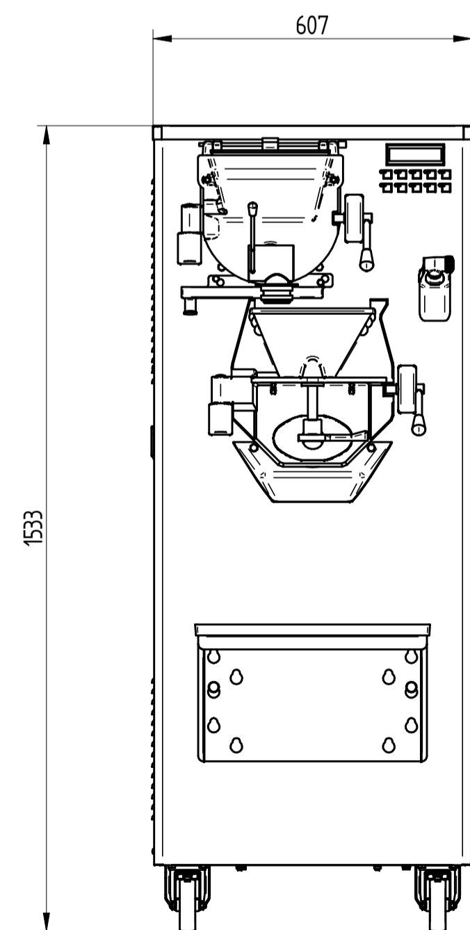
FRONT VIEW
